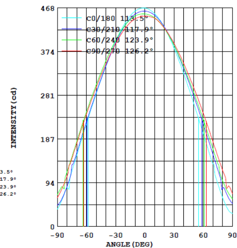
LUMINOUS INTENSITY DISTRIBUTION
