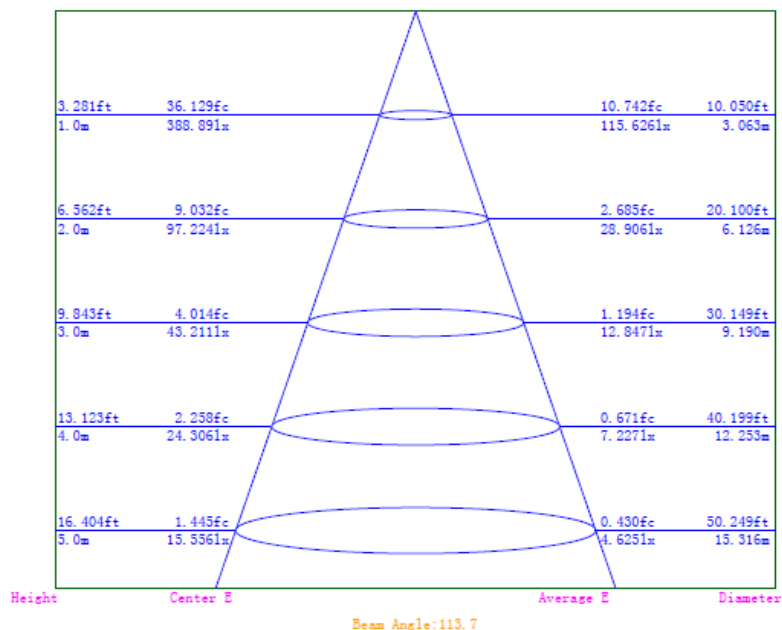
Illuminance-Distance Curve
