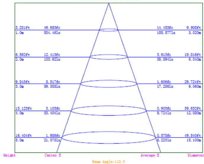
Illuminance-Distance Curve
