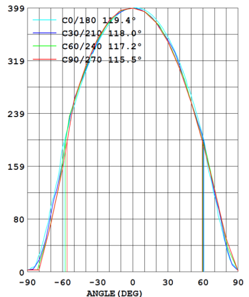
LUMINOUS INTENSITY DISTRIBUTION
