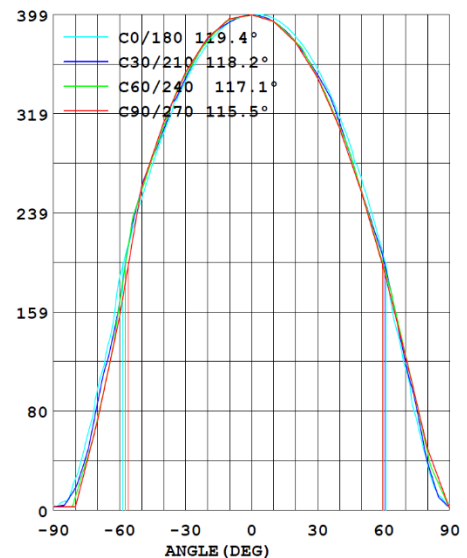
LUMINOUS INTENSITY DISTRIBUTION
