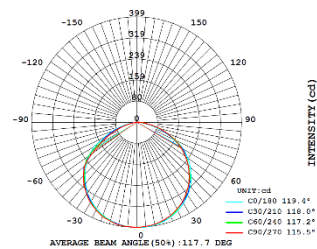
LUMINOUS INTENSITY DISTRIBUTION
